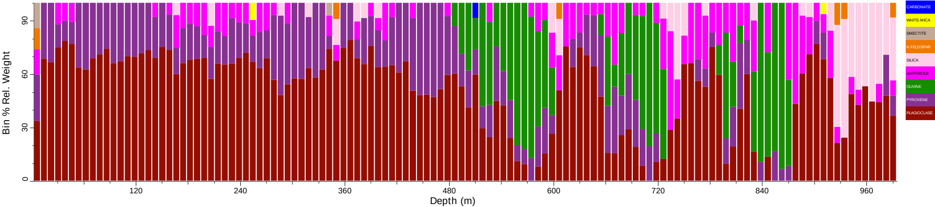
SMD161_tsg_tir: Spatial Summary (Bin=8 MinBin=5% ujCLST 7.08)
