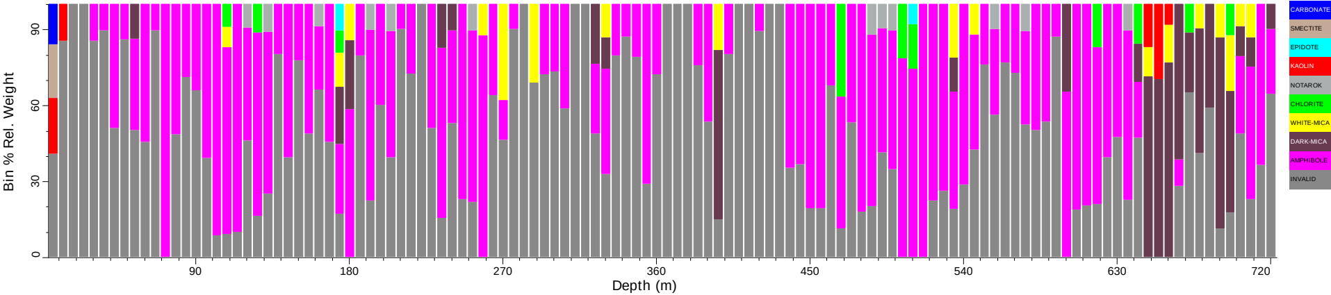
SMD184_tsg_tir: Spatial Summary (Bin=6 MinBin=5% sjCLST 7.08)
