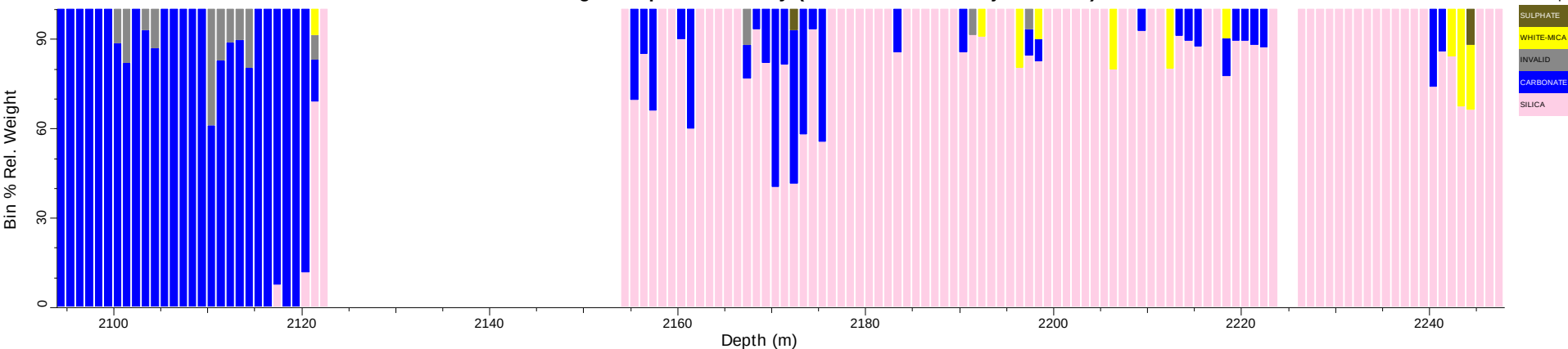
Sunset1_tsg_tir: Spatial Summary (Bin=1 MinBin=5% ujCLST 7.08)
