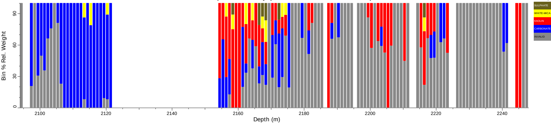
Sunset1_tsg_tir: Spatial Summary (Bin=1 MinBin=5% ujCLST 7.08)
