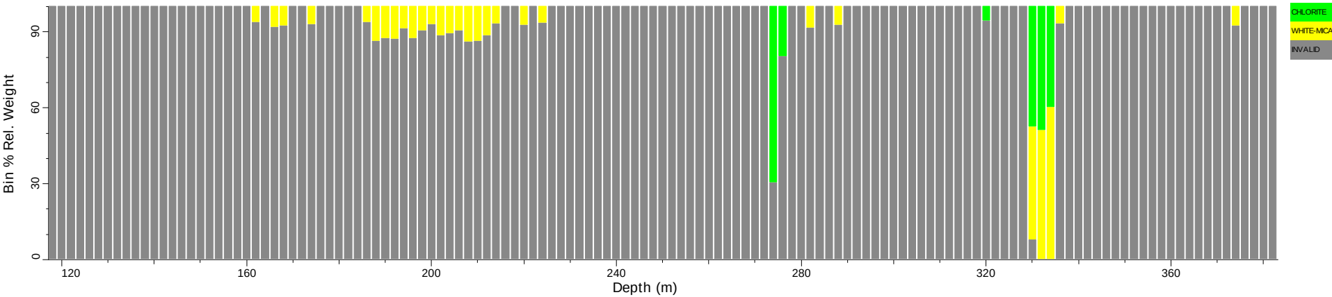
TCDP2_tsg_tir: Spatial Summary (Bin=2 MinBin=5% ujCLST 7.08)
