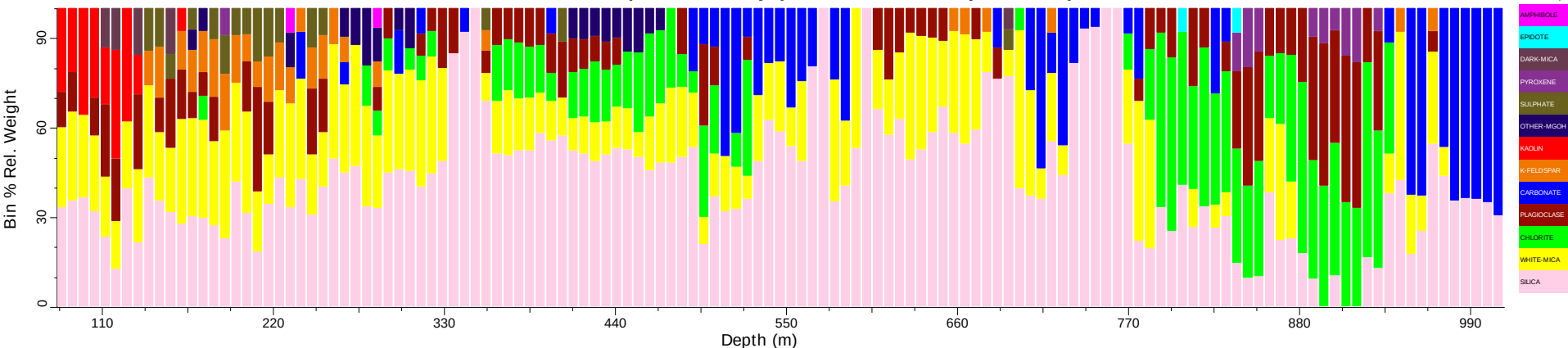
THD001_tir: Spatial Summary (Bin=7 MinBin=5% sjCLST 7.08)
