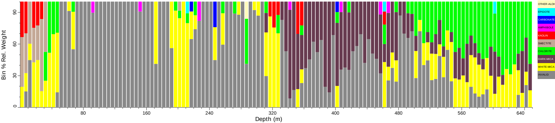
THDD024_tsg_tir: Spatial Summary (Bin=5 MinBin=5% sjCLST 7.08)
