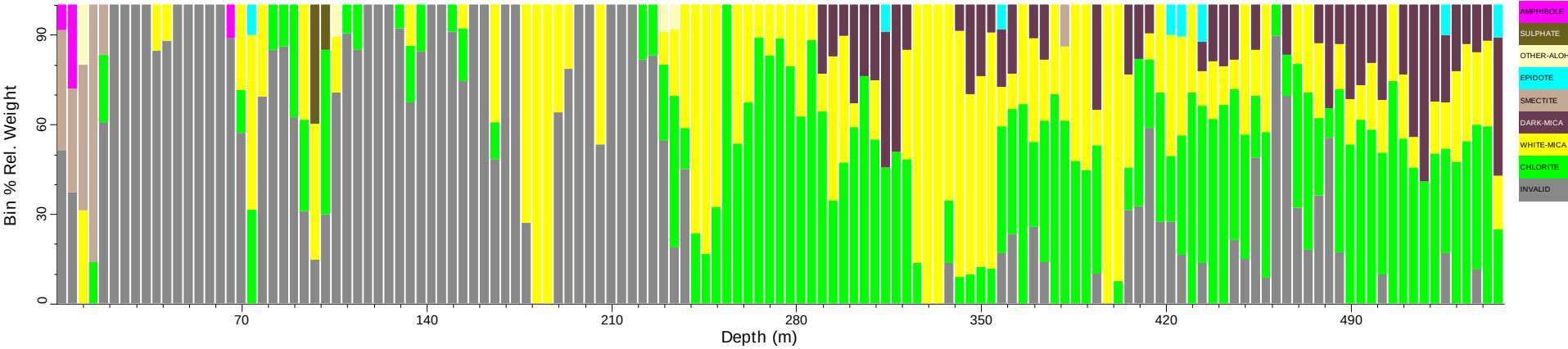
THDD025_tsg_tir: Spatial Summary (Bin=4 MinBin=5% sjCLST 7.08)
