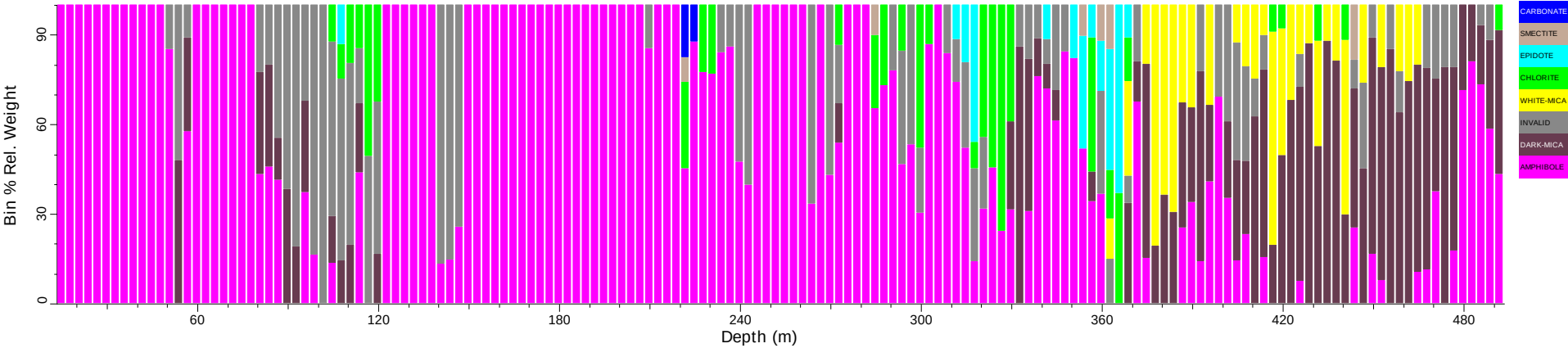
TOR01_tsg_tir: Spatial Summary (Bin=3 MinBin=5% sjCLST 7.08)
