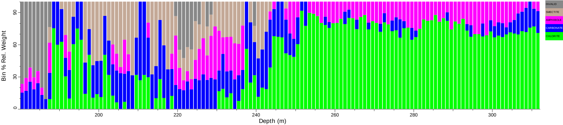
UEC07_tsg_tir: Spatial Summary (Bin=1 MinBin=5% ujCLST 7.08)
