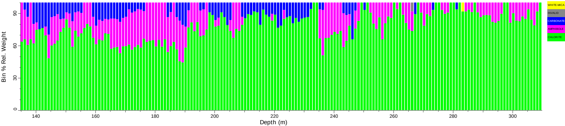
UEC08_tsg_tir: Spatial Summary (Bin=1 MinBin=5% ujCLST 7.08)
