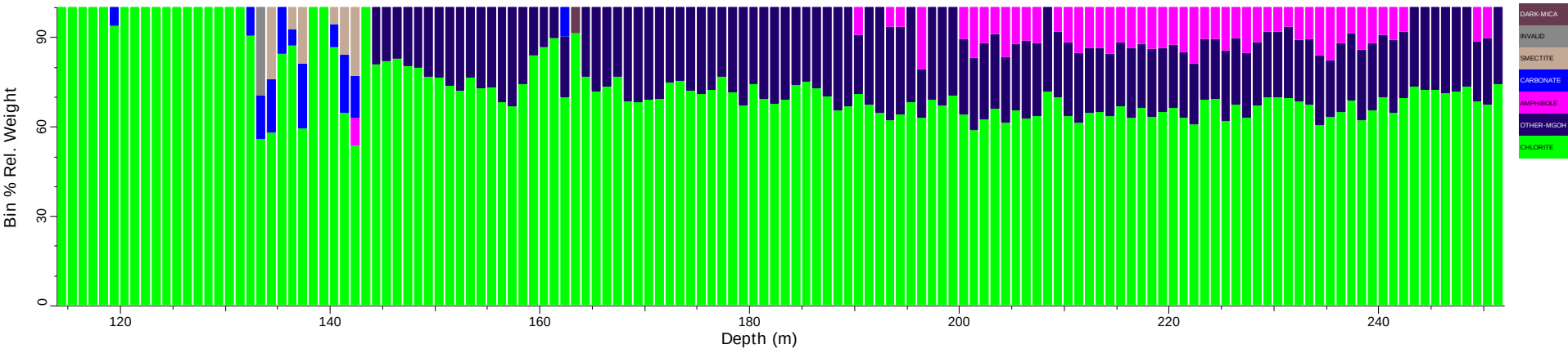
UEC09_tsg_tir: Spatial Summary (Bin=1 MinBin=5% ujCLST 7.08)
