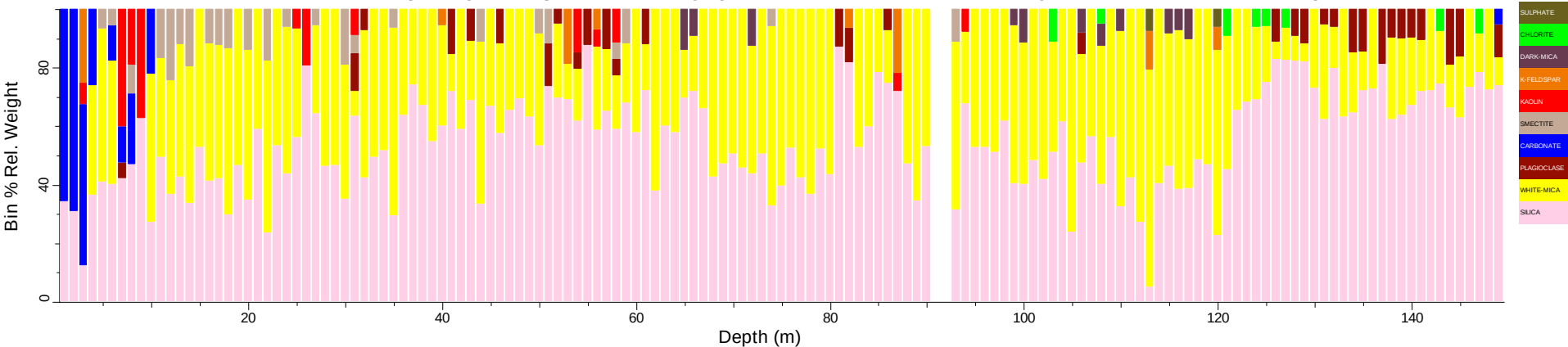
WBRC2201_chips_tsg_tir: Spatial Summary (Bin=1 MinBin=5% Un-edited sjCLST 7.08, Mineral Subset)
